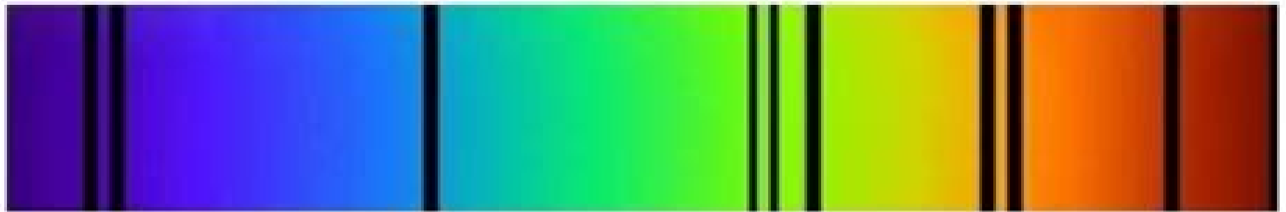
Blueshifted spectrum
