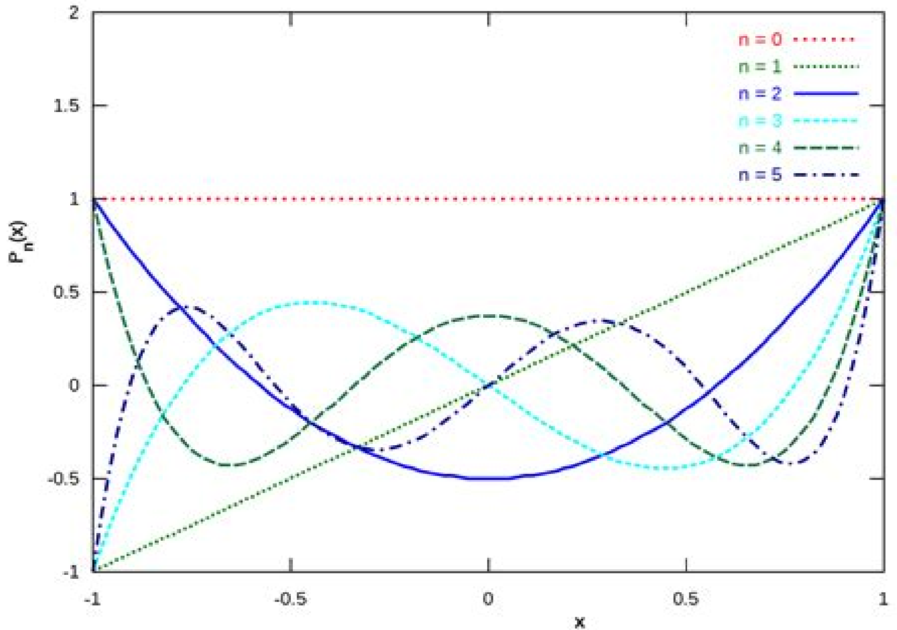
Legendre Polynomials
