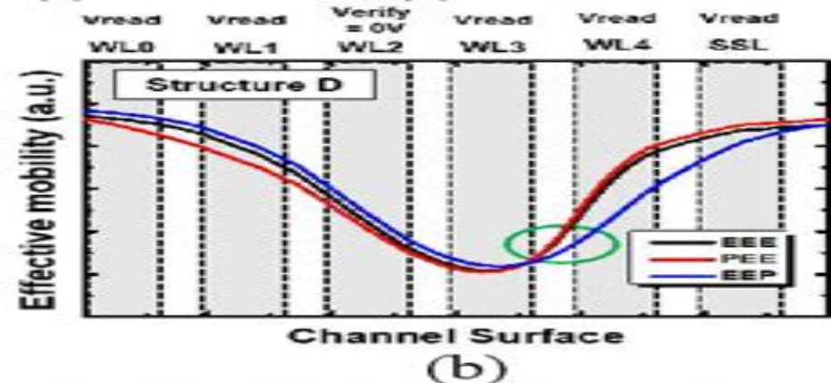
Figure 5. Electron mobility at channel surface during read operation (a) structure A, (b) structure D.
