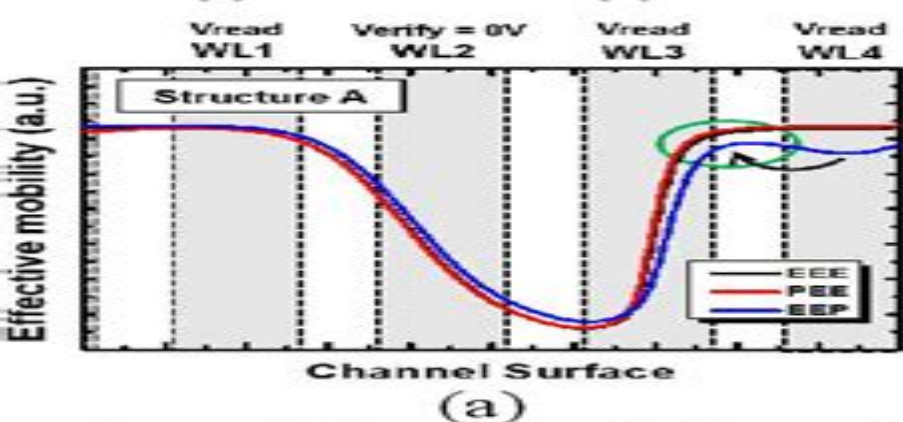
Figure 5. Electron mobility at channel surface during read operation (a) structure A, (b) structure D.
