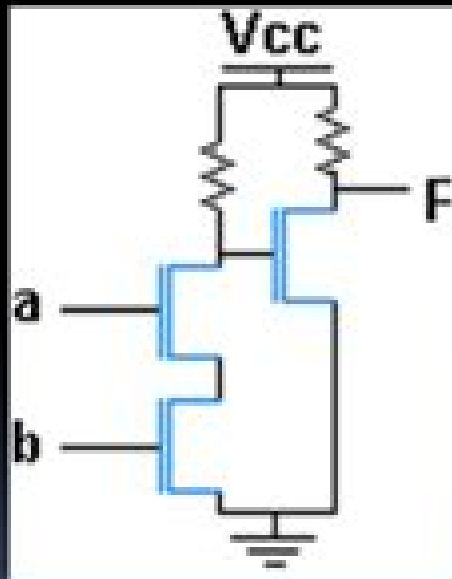
NMOS AND gate
