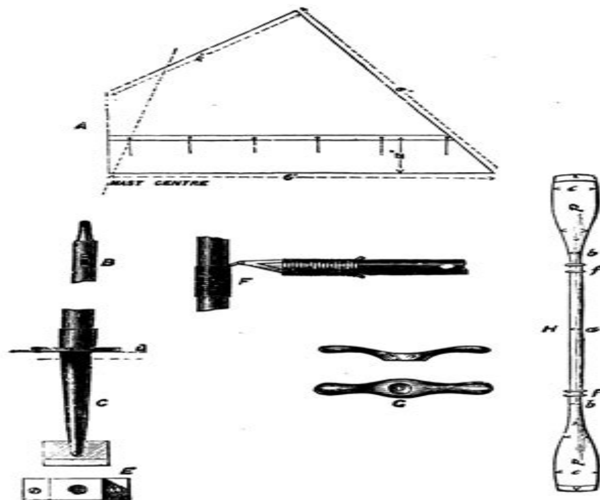
FIG. 47. SAIL, PADDLE, AND FITTINGS OF ROB ROY CANOE.
