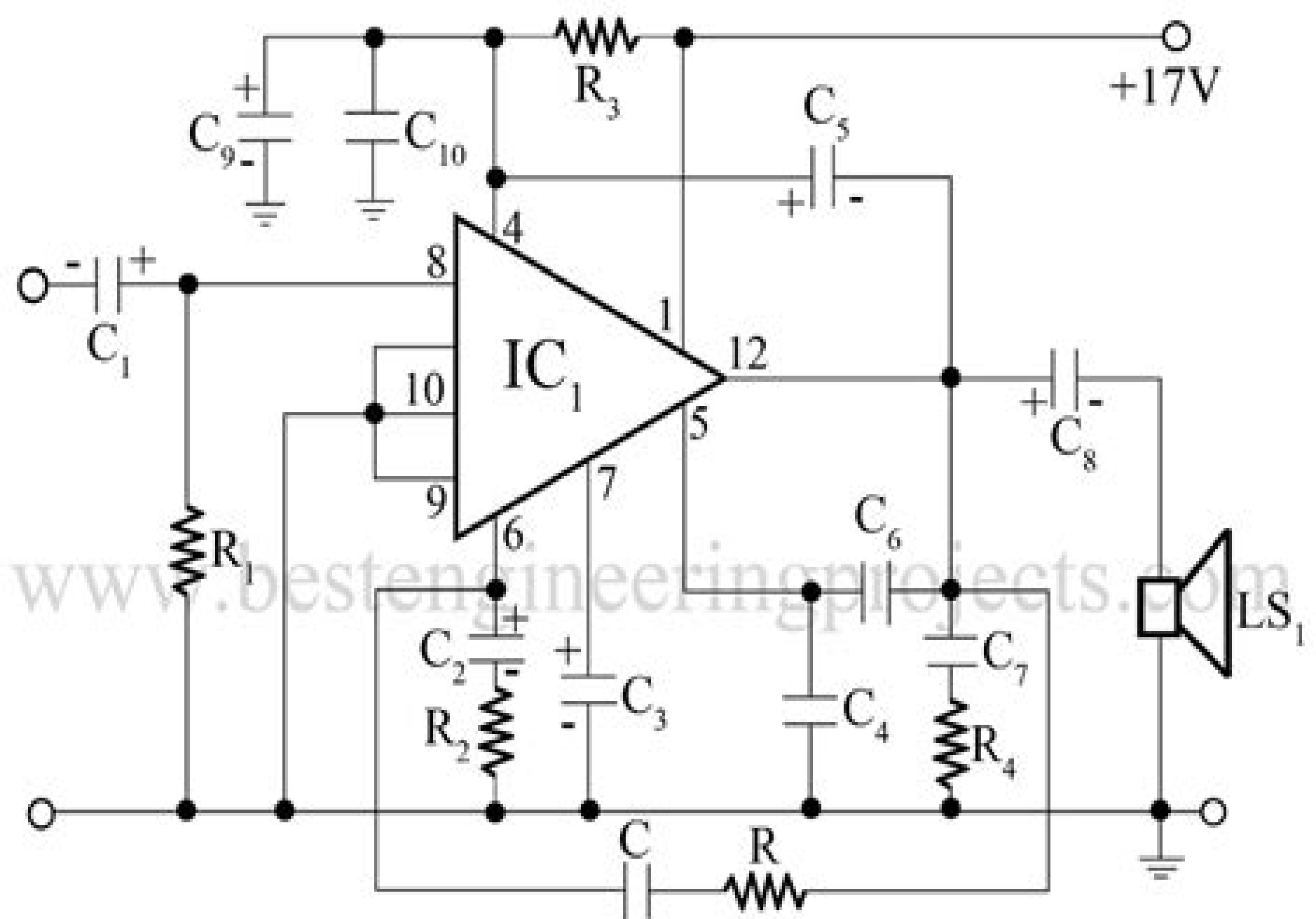
Figure 1: Circuit Diagram of Audio Amp Using TBA810 IC
