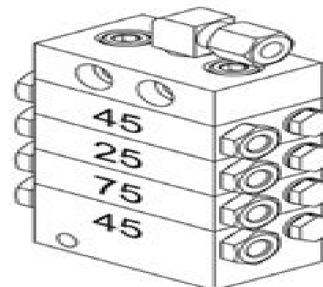
Dimension drawing:
