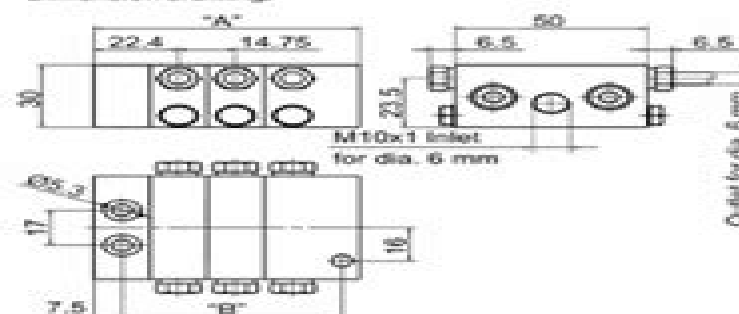
Dimension drawing:
