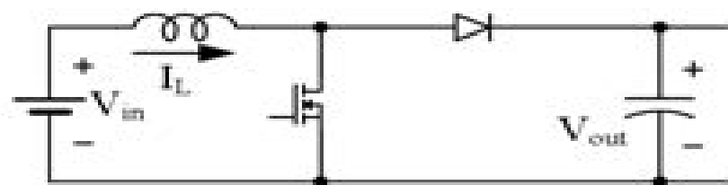
(c) Boost converter
