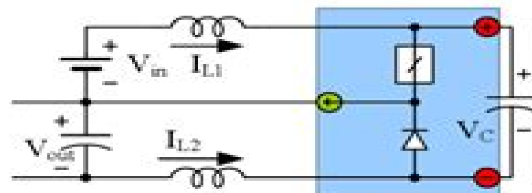
(h) P-cell Cuk converter
