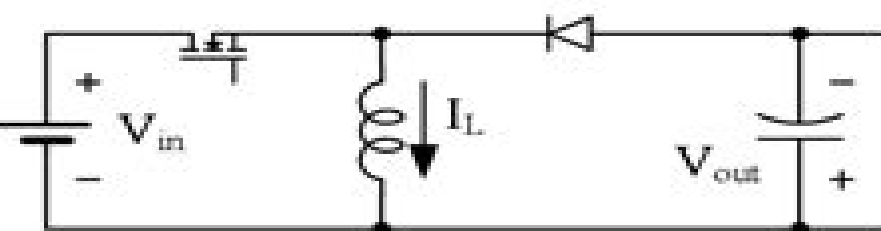
(e) Buck-boost converter
