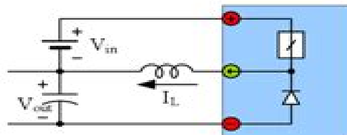
(f) P-cell buck-boost converter
