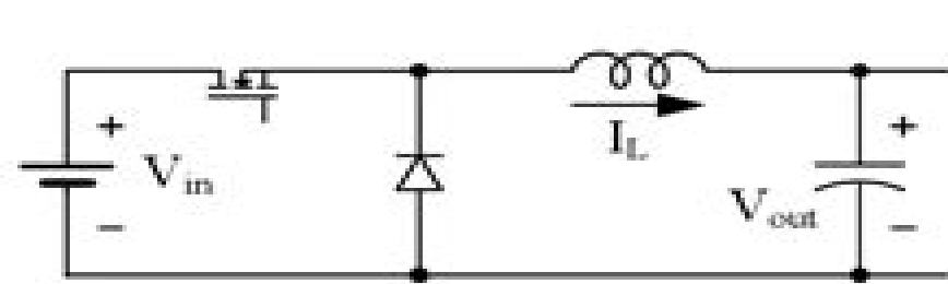
(a) Buck converter
