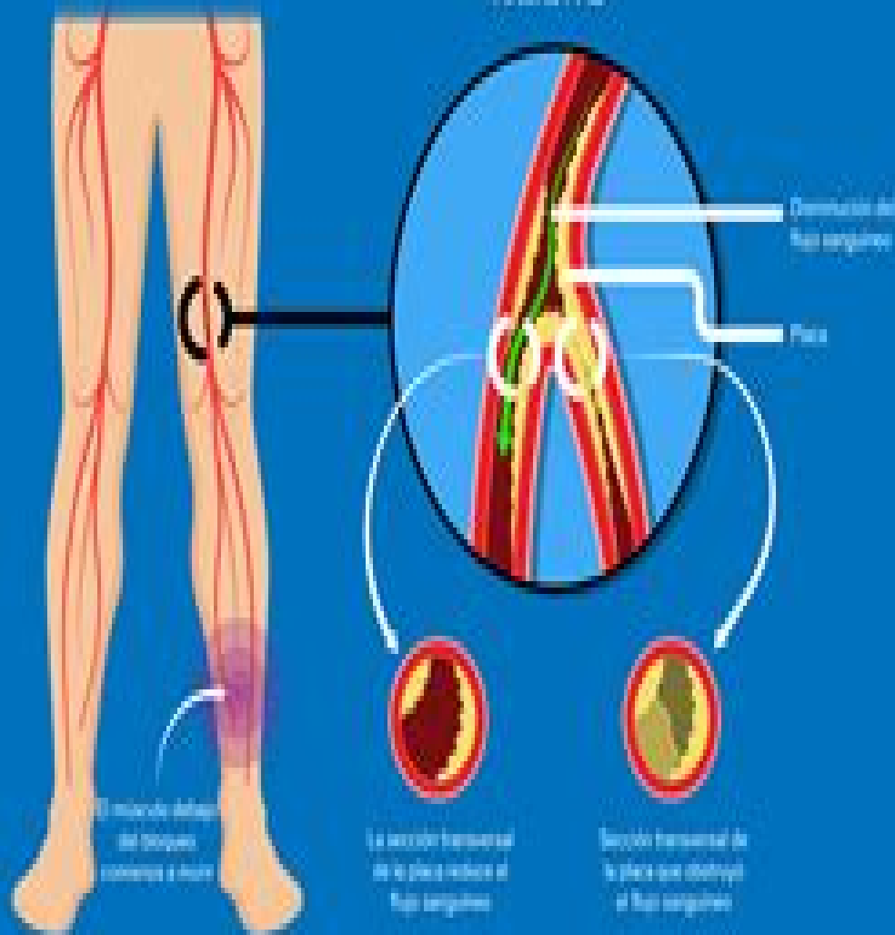
Arteria PAD
