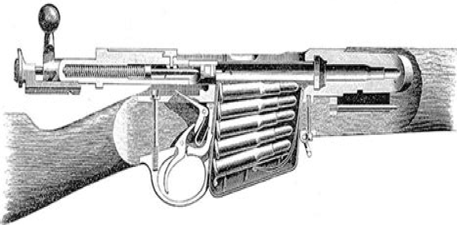
Sectional View, Magazine Charged and in Position.
