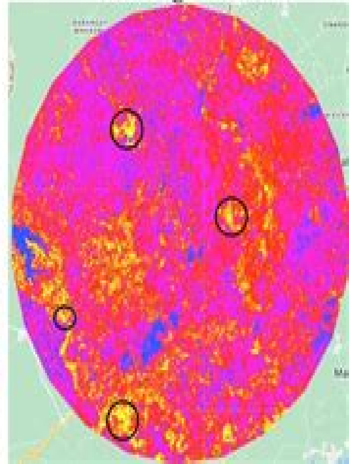
Iron oxide & Hydroxyl Bearings minerals
