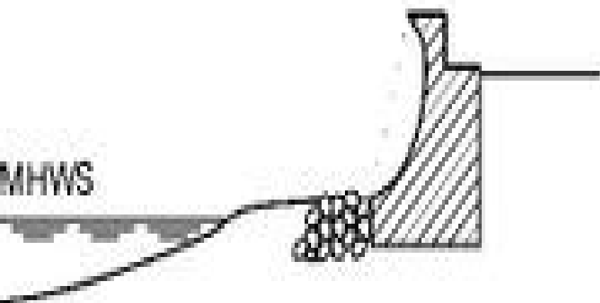
Curved concrete seawall
