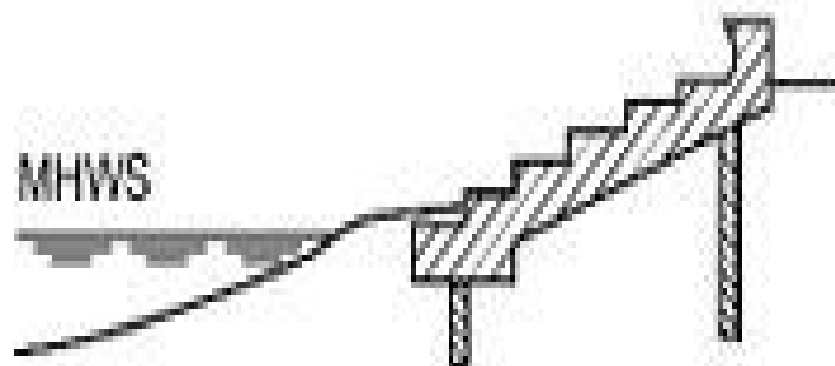
Stepped and curved concrete seawall
