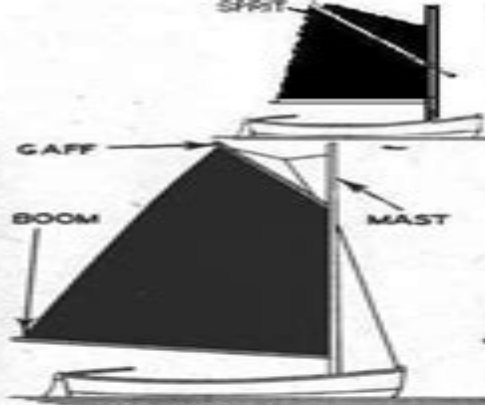
GAFF RIG
