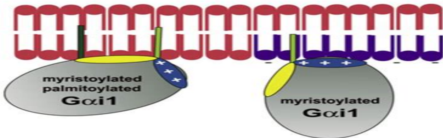
Myristoylated Palmitoylated
