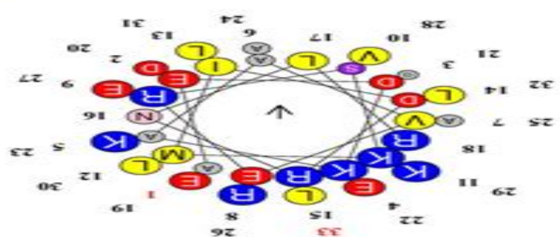
Myristoylated Palmitoylated
