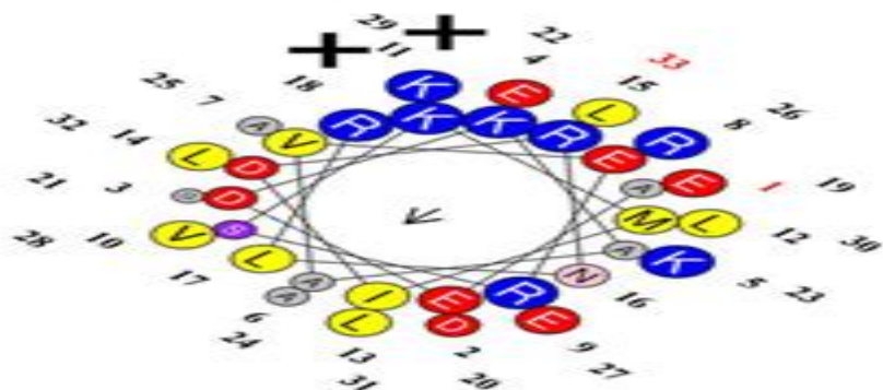
Myristoylated
