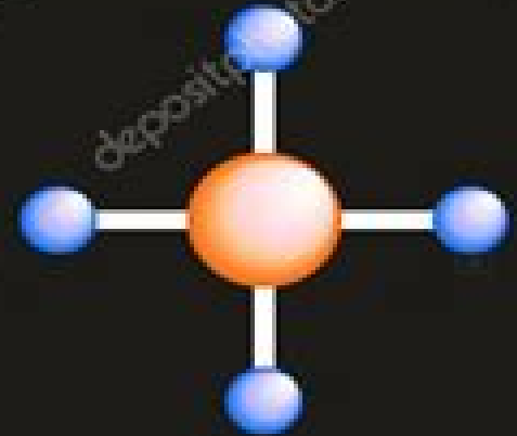
Square Planar
