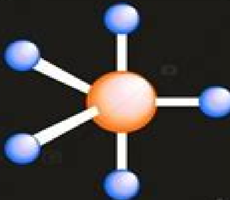
Trigonal Bipyramidal
