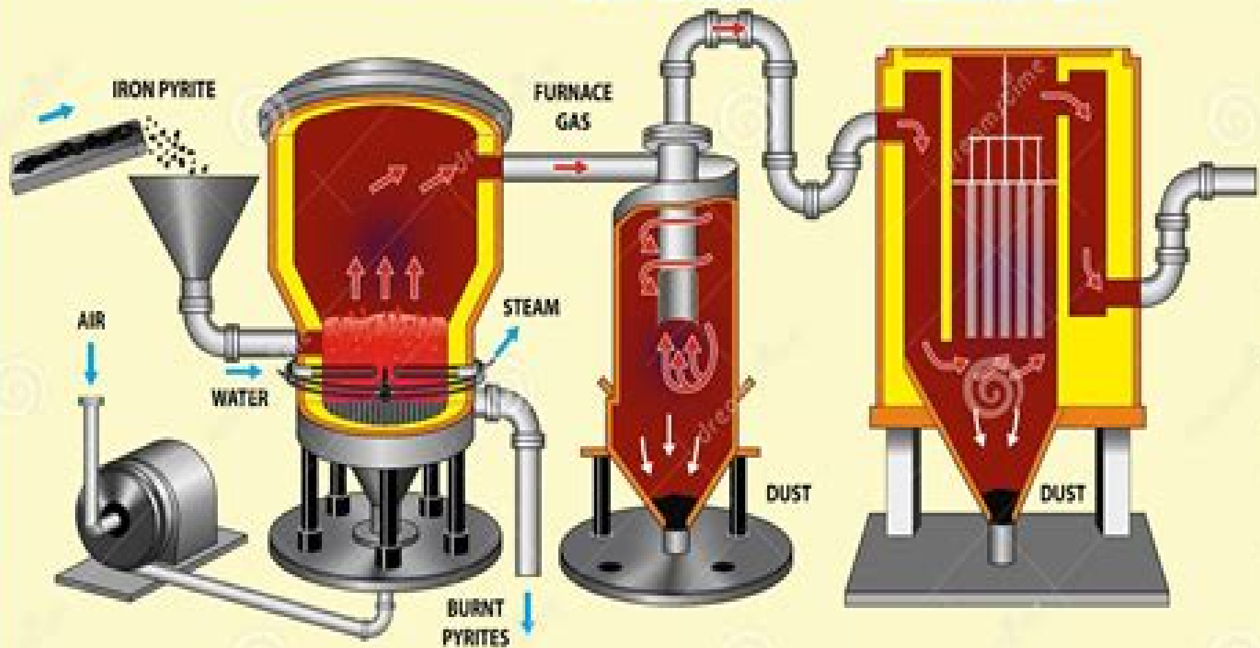
CYCLONE DUST COLLECTOR
