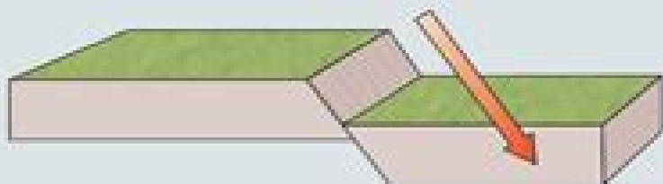
(a) Displacement occurs when a block of rock moves from one place to another.
