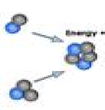
Nuclear Fusion
