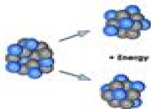
Nuclear Fission
