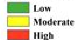
Legend Drought risk (2022)
