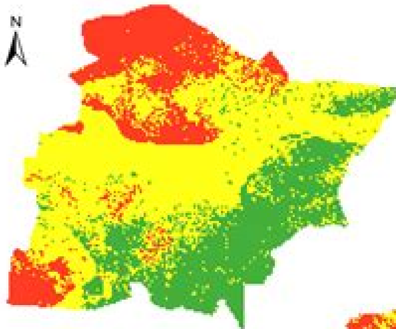
Legend Drought risk (2002)
