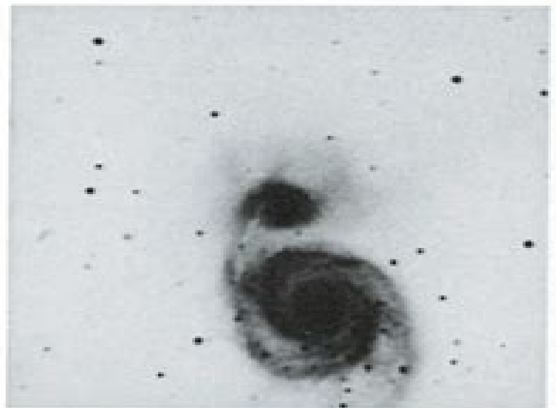
NGC5195
