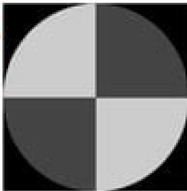
Recovered albedo
