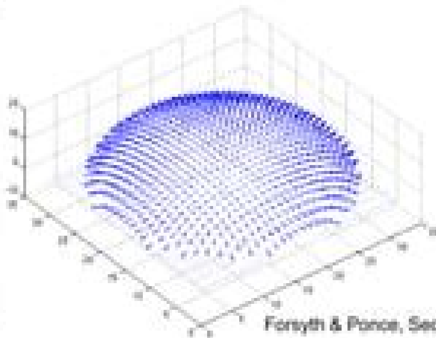
Recovered normal field
