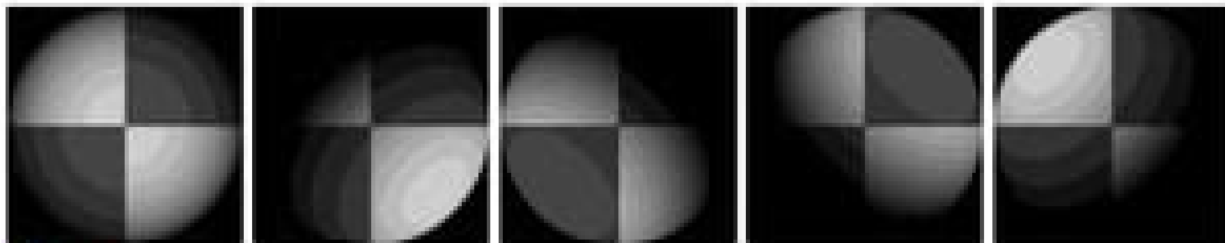
Recovered albedo
