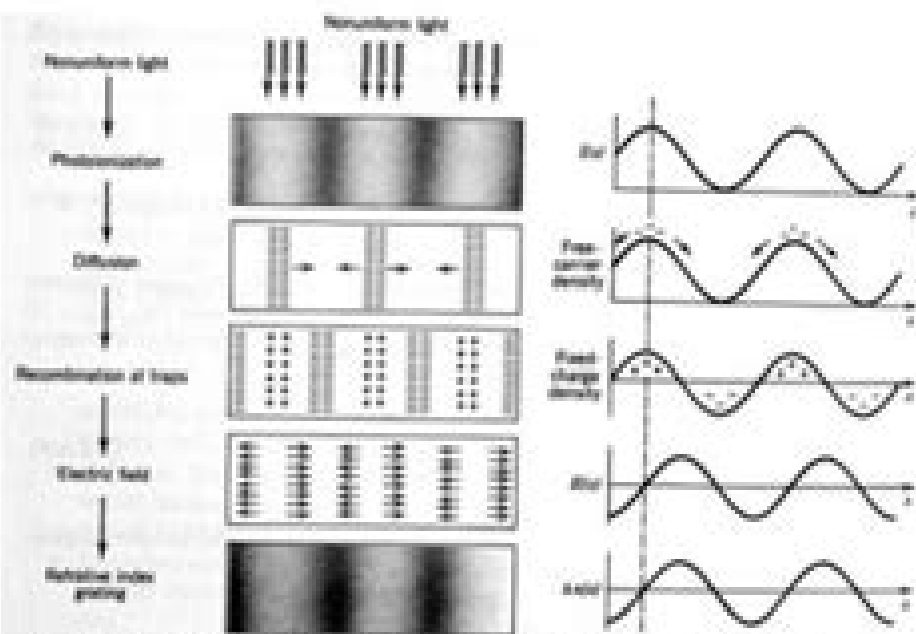
Figure 18.4-2 Response of a photorefractive material to a sinusoidal spatial light pattern.
