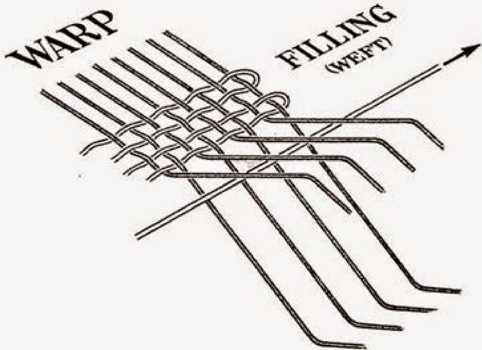
Fig: Picking (Weft insertion)
