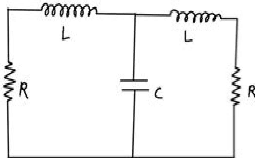
Fig. Lumped Network
