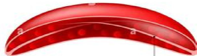
Long polymerized sickle haemoglobin (HbS)
