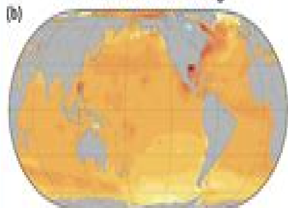
SSP1-2.6 median change
