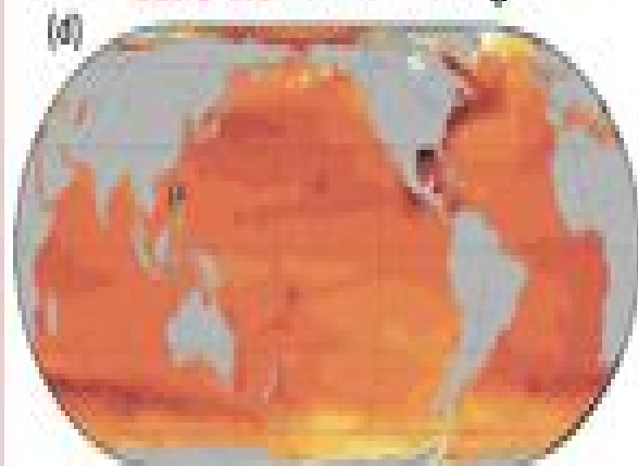
SSP3-7.0 median change
