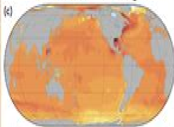
SSP2-4.5 median change
