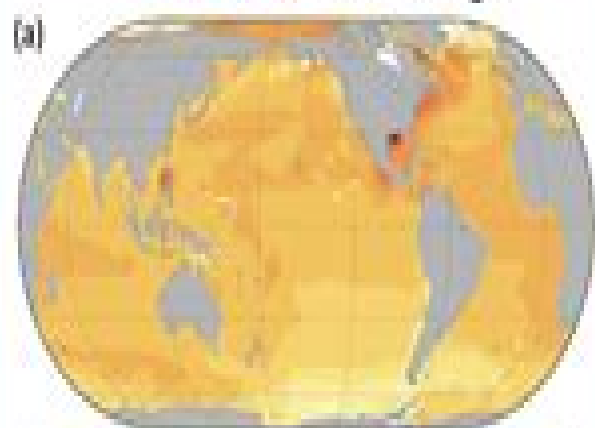
SSP1-1.9 median change
