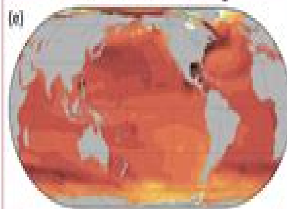
SSP5-8.5 median change
