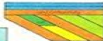
glacier
