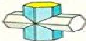
twin crystal
