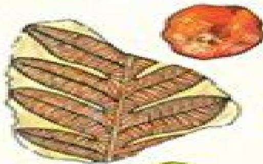
fossil plants
