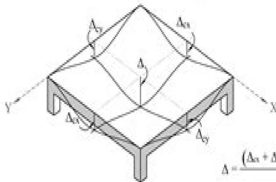
c) Combined Bending
