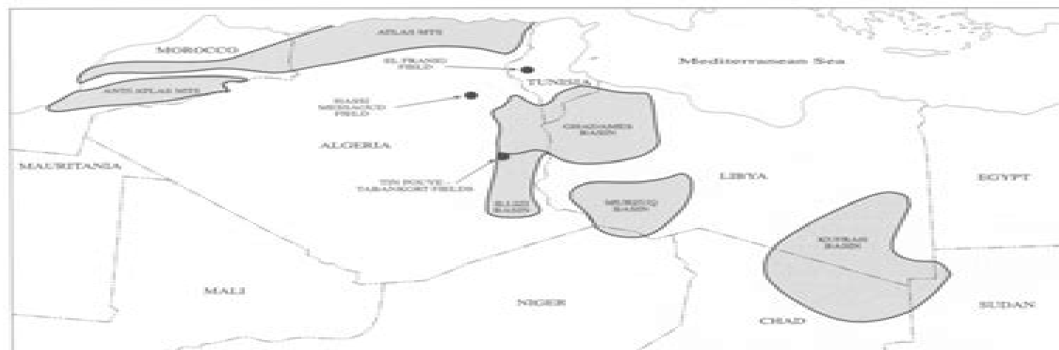
Fig. 1. North Africa locality map.
