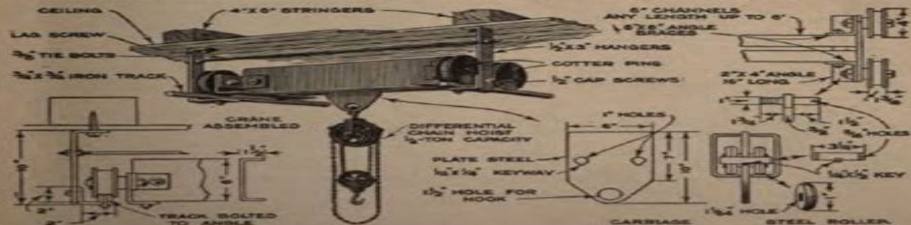
A Light-Running Crane, Which will Add Greatly to the Ease of Handling Materials in a Small Shop. Is Easily Constructed of Available Materials
