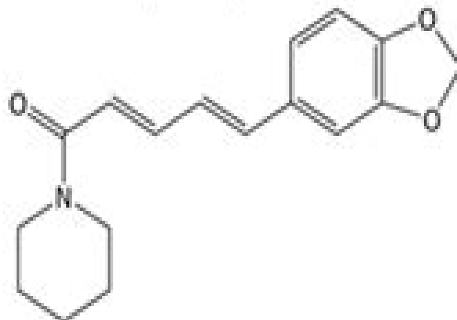
2-Acetylpyridine [14.038]
