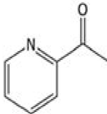
2-Acetylpyridine [14.038]
