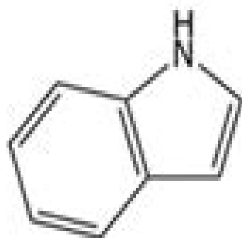
3-Ethylpyridine [14.061]
