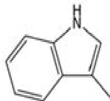
3-Methylindole (skatole) [14.004]
