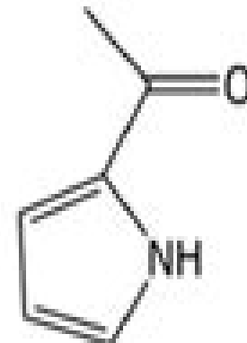
2-Acetylpyrrole [14.047]
