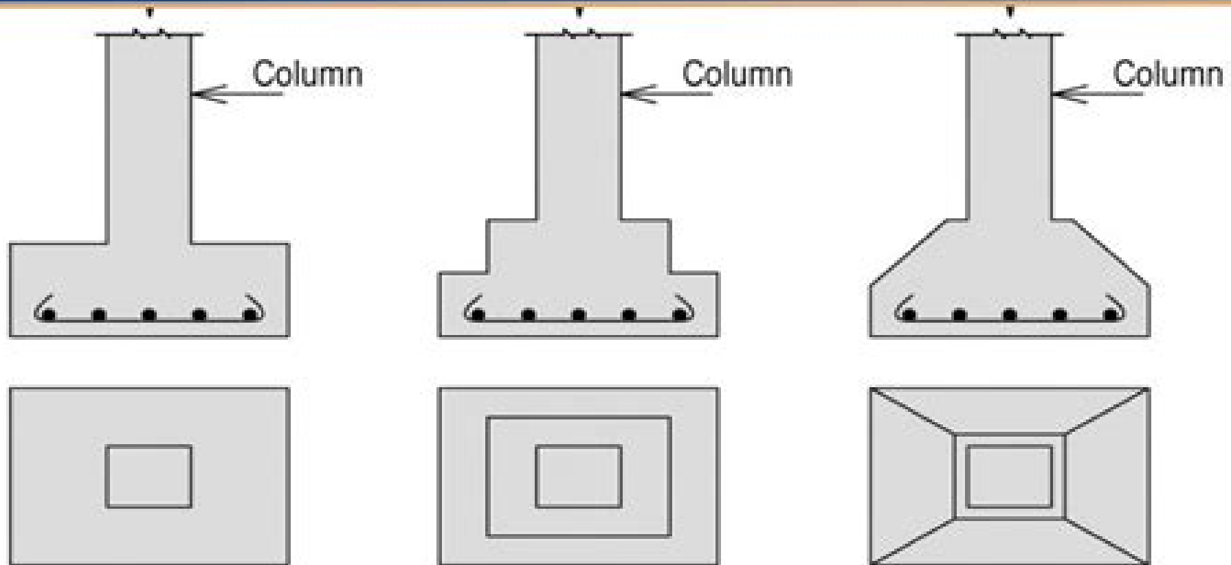
Shallow Foundation
