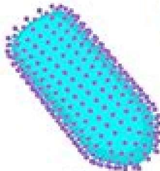
Rabies 180x80nm
