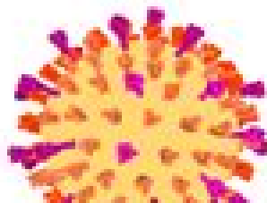
Measles 150nm
