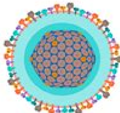
Herpes virus 200nm
