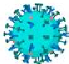
Influenza virus 100nm
