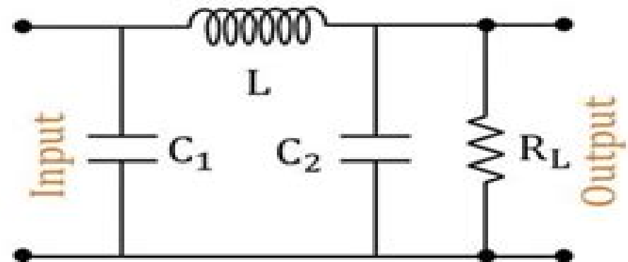
CLC or \pi Filter
