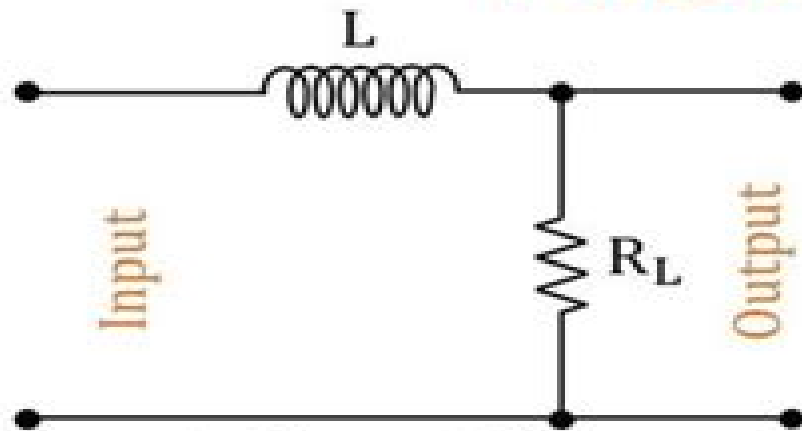
Inductor Filter
