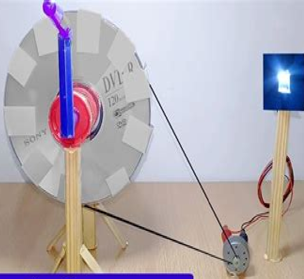
Electric Generator
