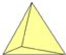
Tetraeder
