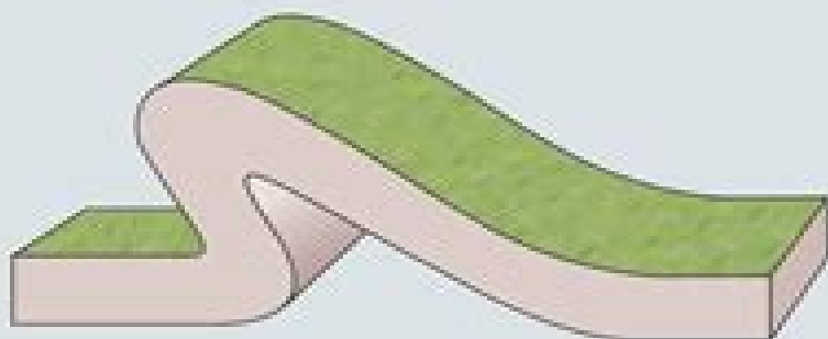
(c) Distortion occurs when rock changes shape. The development of a fold represents one type of distortion.
