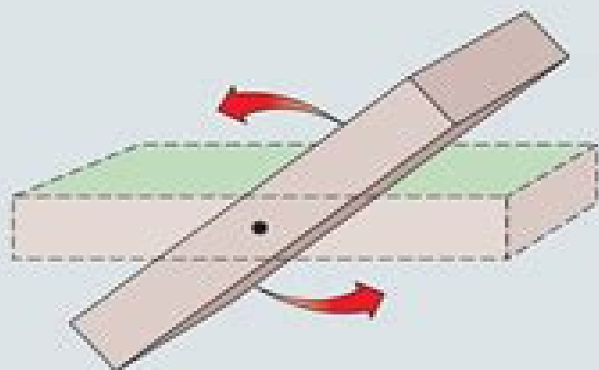
(b) Rotation occurs when a body of rock undergoes tilting.
