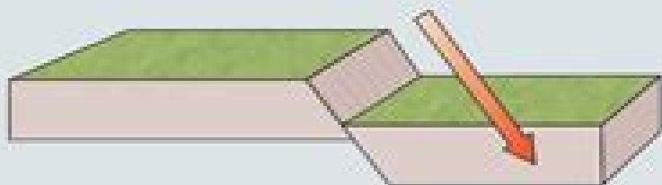
(a) Displacement occurs when a block of rock moves from one place to another.
