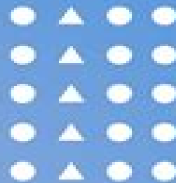
SIMILARITY
