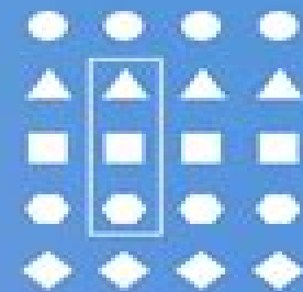
COMMON REGION
