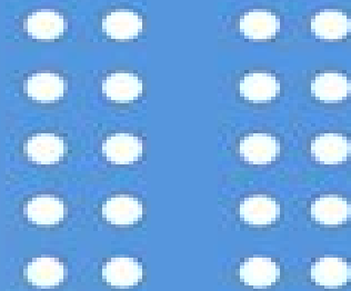
PROXIMITY
