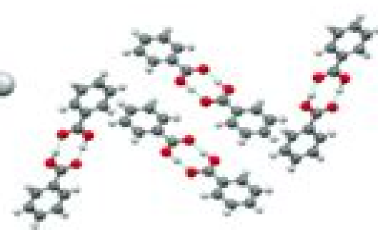
Organic compound
