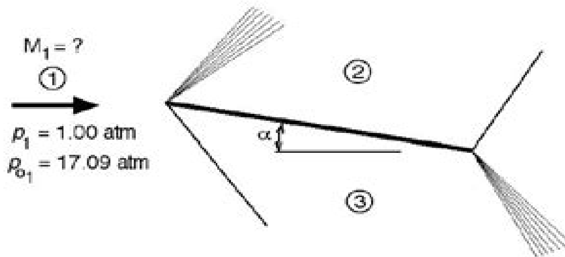
Figure 1. Flat plate aerofoil
