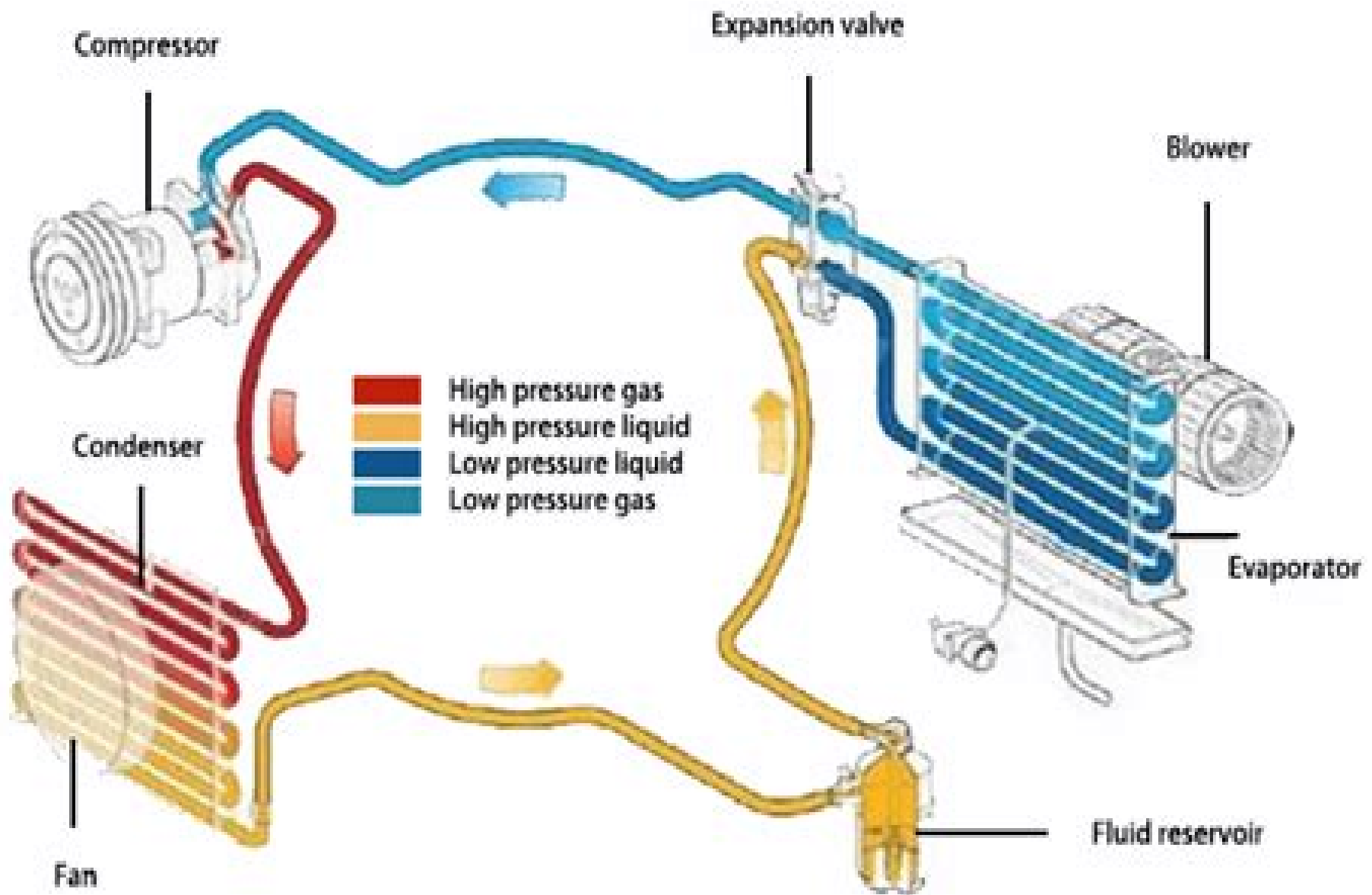
Air Conditioning System Schematic
