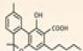
Cannabinolic acid CBNA
