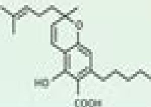
Cannabichromenic acid CBCA
