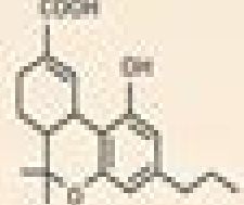
Tetrahydrocannabivarin carboxylic acid THCVA
