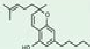
Cannabichromene CBC
