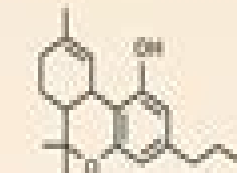
Tetrahydrocannabivarin THCV
