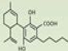
Cannabinolic acid CBDA
