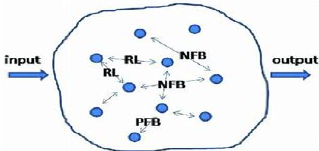
Figure 5. Feedback base regulatory patterns of a biological system. NFB—negative feedback; RL—reciprocal links; (PNR). PNR are observed in various systems on molecular, cell and organ levels.
