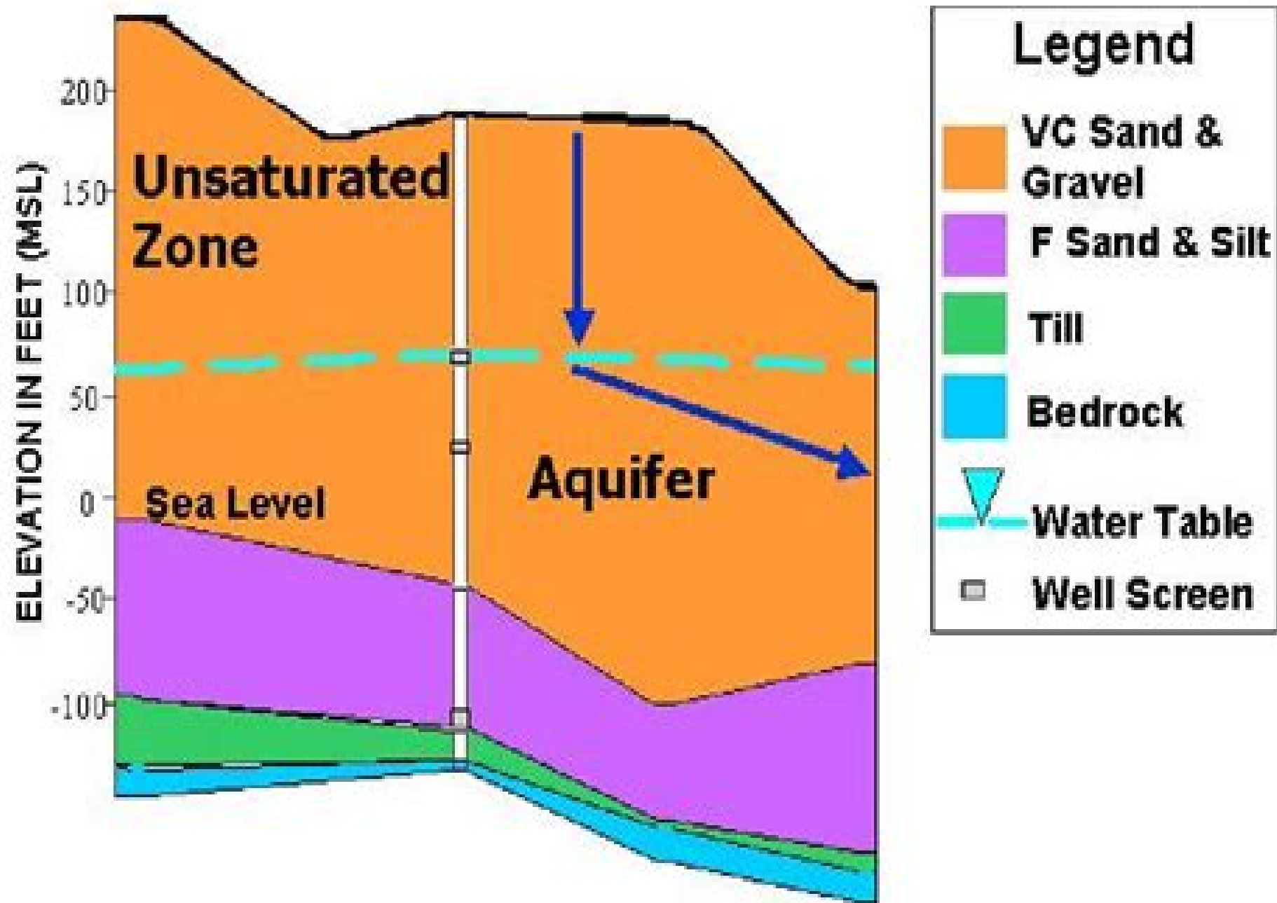
Figure 1. Generalized Lithologic Cross-Section for the site.
