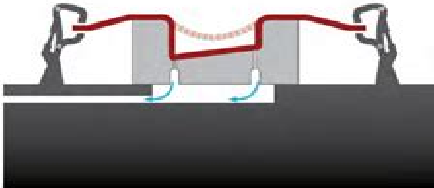
3 Air is evacuated from the mold, pulling the plastic onto mold surface
