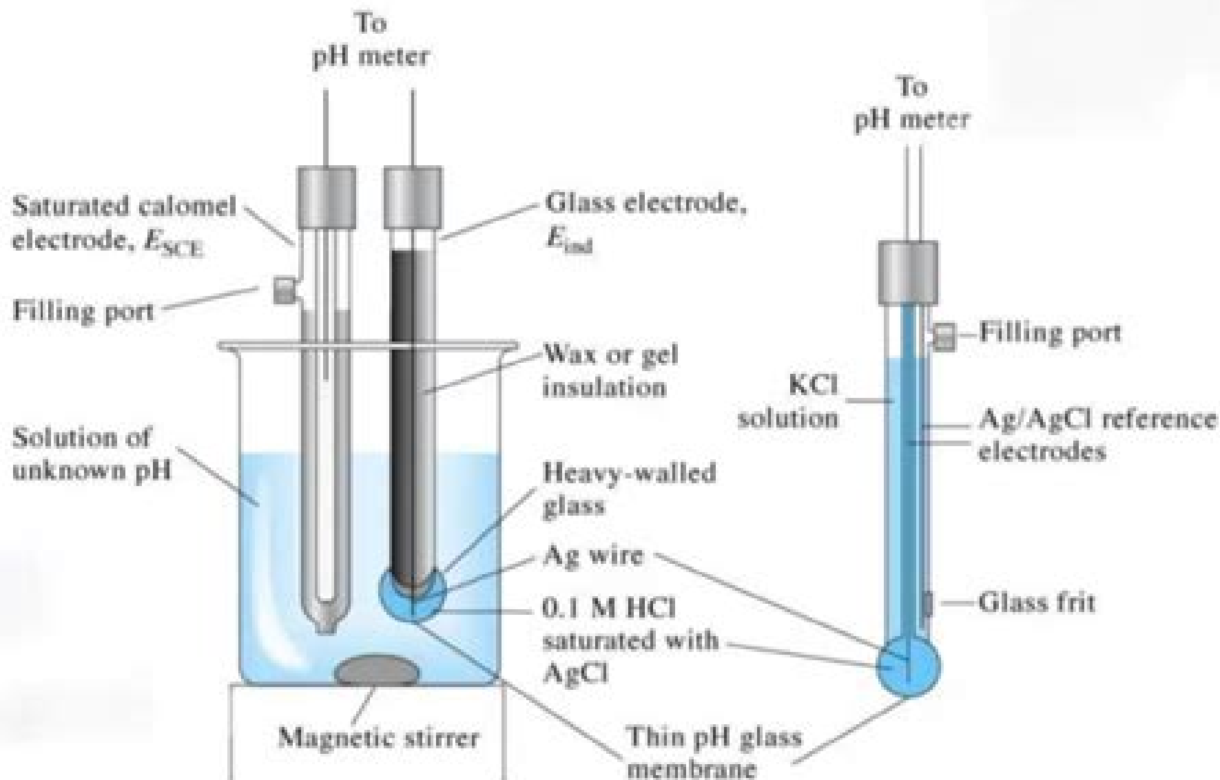
Parts of a pH meter
