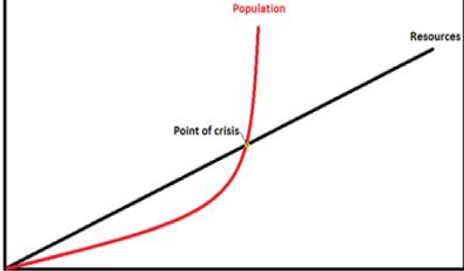
Malthus' Basic Theory
