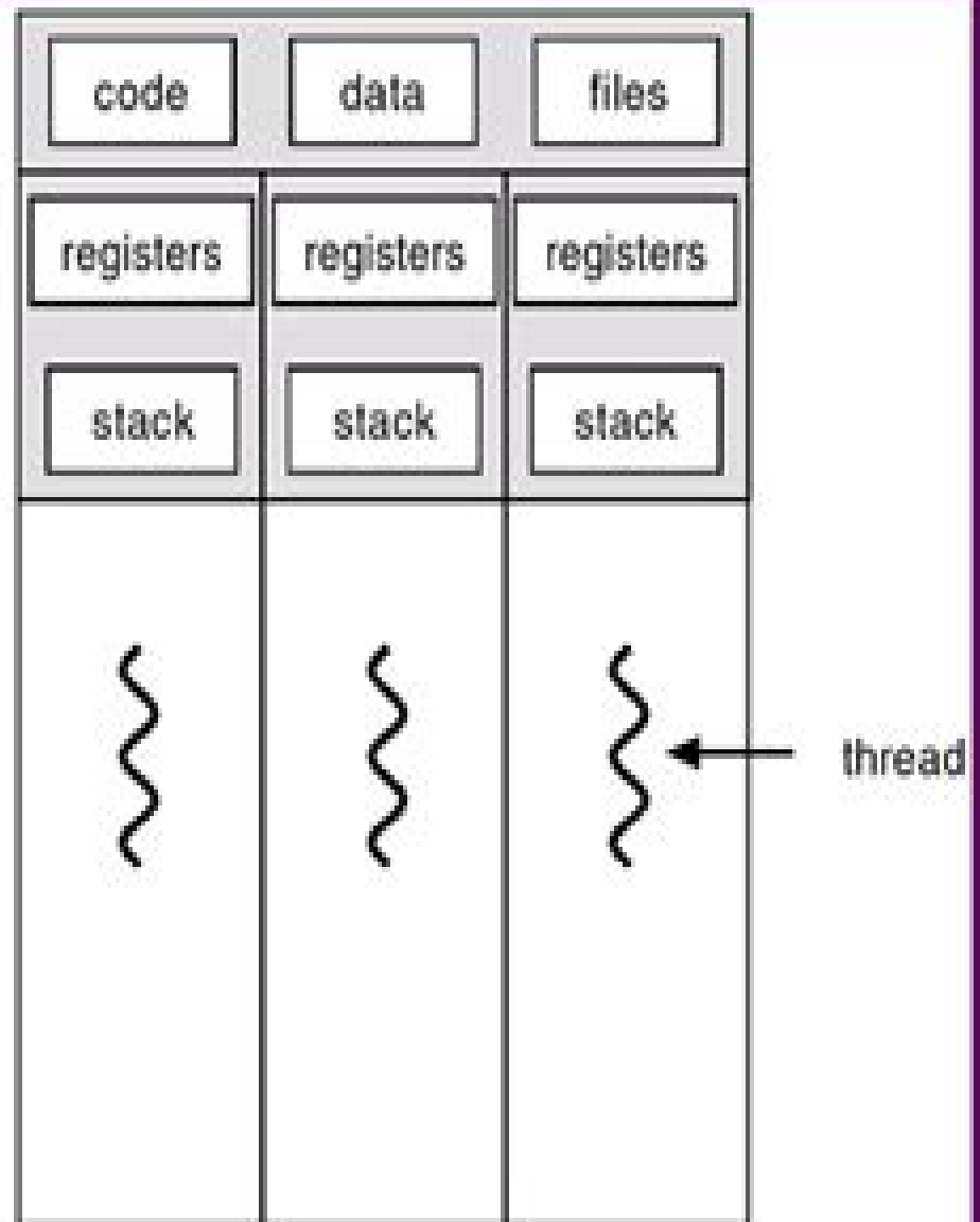
multithreaded
