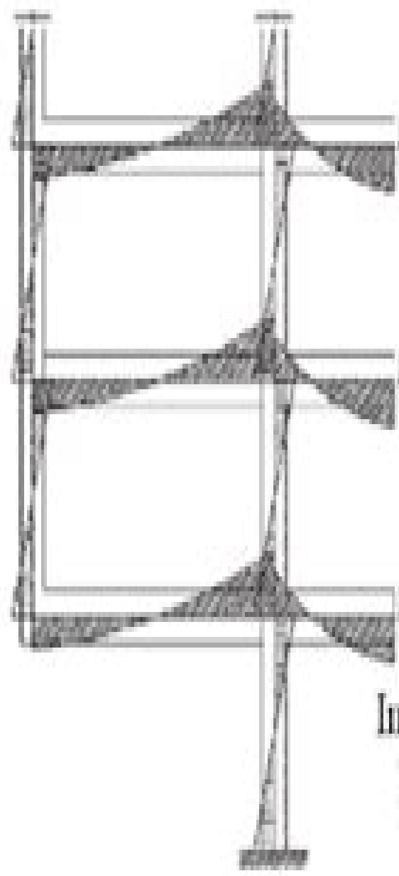
b) B.M.D after column loss
