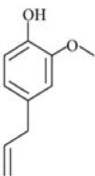
Eugenol
