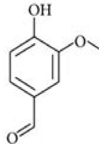
Vanillin
